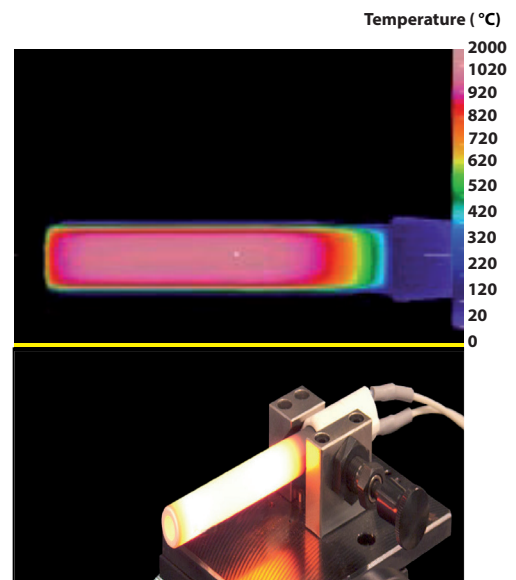
Heat distribution
